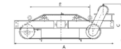
Installation Sketch Map (declining form)
