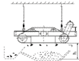
Installation Sketch Map (aclinic form)
