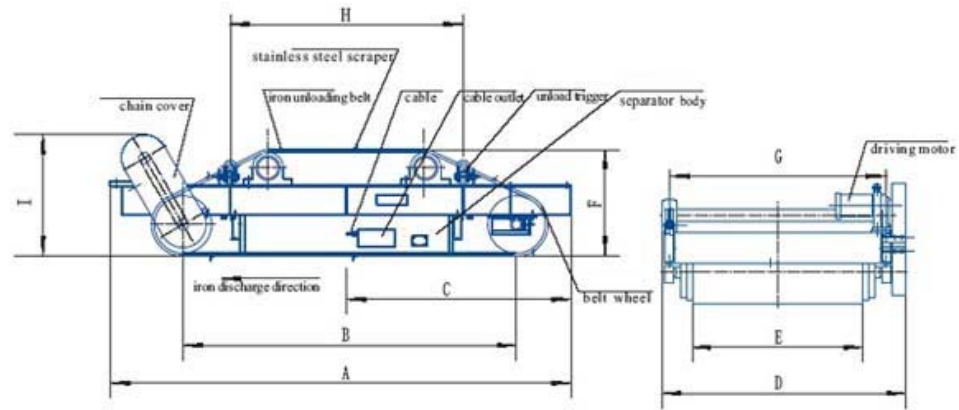
overall dimension drawing
