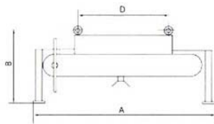
Overall Dimension Drawing
